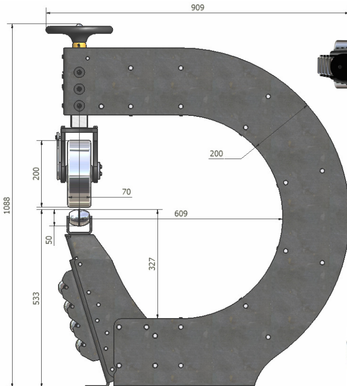
EW10000 - General Dimensions
